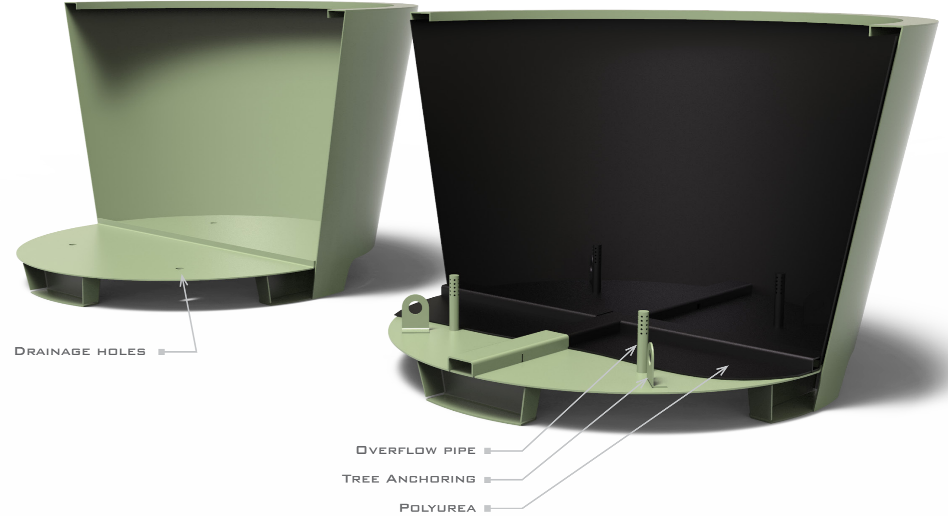
STANDARD PLANTER
